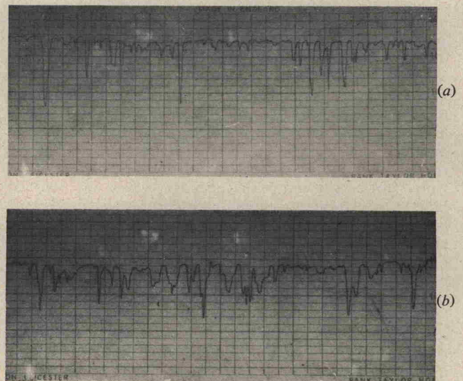
Fig. 5 Surface profile of the extruded product: (a) At 8.89 cm/min drawing speed; (b) at 82.5 cm/min drawing speed.
