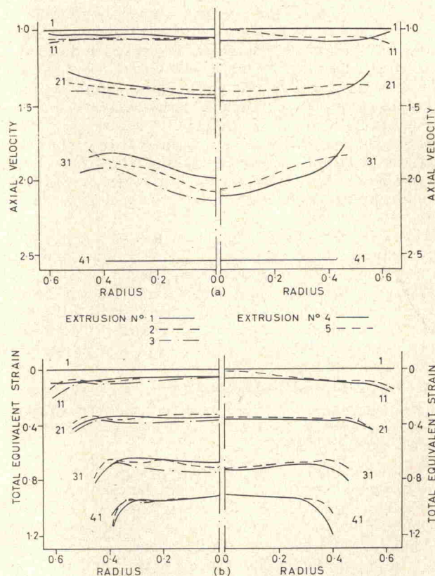
Fig. 4 Axial velocity and total equivalent strain distribution in the deforming region: (a) Axial velocity; (b) total equivalent strain. Extrusion numbers refer to test numbers given in Table I. Numbers adjacent to the curves refer to axial co-ordinates in Fig. 2. Radius in cm.
